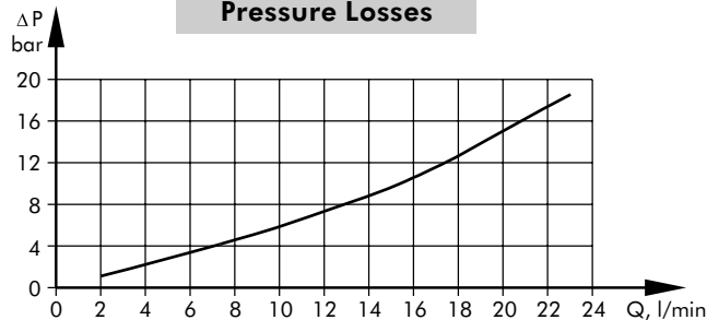
Pressure Losses
